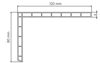
W 9050 Pervaz Profili Sill Joint Extension Profile Ağırlık / Weight : 0.820 kg / mt
