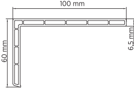
W 9020 Pervaz Profili Sill Joint Extension Profile Ağırlık / Weight : 0.720 kg / mt
