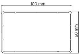
W 9010 100 x 60 Kutu Profili 100x60 Corner Profile Ağırlık / Weight : 0.990 kg / mt
