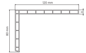
W 9050 Pervaz Profili Sill Joint Extension Profile Ağırlık / Weight : 0.820 kg / mt
